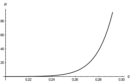
Fig. 3. R_{A/NA} providing that r = 0.9, q \in [0.2, 0.3] .
